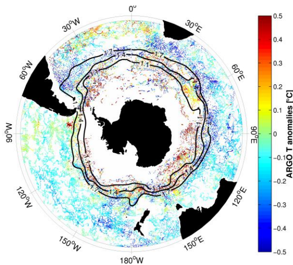
Figure 2: The dots show the distribution of 52,447 Argo profiles used to calculate the deviations of Argo potential temperatures averaged over the neutral-density layer 26.9–27.7 from the climatological mean. Dark curves are contours of climatological dynamic height giving an approximate representation of ACC position. The plot indicates the coverage of the Southern Ocean obtained in the first few years of the Argo program. (From [6]).
