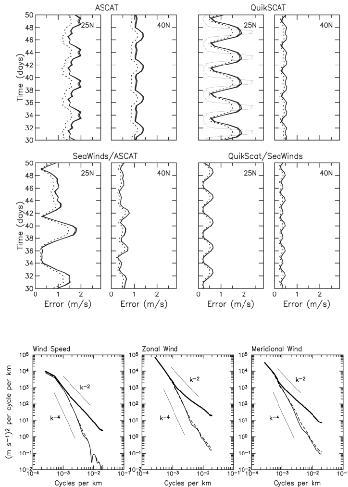
Figure 2. Upper panels: Time series of the RMS mapping errors of meridional (solid lines) and zonal (dotted lines) wind estimates constructed at latitudes of 25^\circ\text{N} and 40^\circ\text{N} from various combinations of scatterometer observations with 2^\circ by 2^\circ by 4-day smoothing. The three solid lines correspond to different assumed forms for the spatial autocorrelation function; the small differences show that the results are not strongly sensitive to the details of the spatial autocorrelation function; the most limiting factor for construction of wind fields is the short decorrelation time scale of the surface wind field. (The thin solid line in the QuikSCAT panel is a time series of the RMS (Root-Mean-Square) mapping errors at 25^\circ\text{N} with 2^\circ by 2^\circ by 1.5-day smoothing.) (From [97].) Lower panels: Along-track wavenumber spectra of wind speed and the zonal and meridional wind components in the eastern North Pacific, accumulated over 2004, computed from QuikSCAT observations (heavy solid lines), NCEP (National Centers for Environmental Prediction) analyses (thin solid lines) and ECMWF analyses (dashed lines; the 2004 version had \sim 40\text{km} grid spacing compared to the current \sim 25\text{km} ). Note the drop-off of spectral energy in the two operational forecast models at wavelengths shorter than about 1000 km (wavenumbers higher than about 10^{-3} cycles per km). (From [20].)
